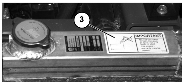
Next to engine radiator filler cap
